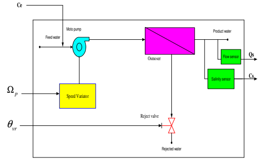
Fig. 4. The desalination unit configuration.
