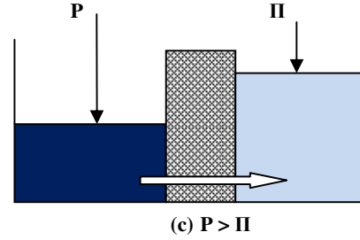
Fig. 2. Principle of the reverse osmosis : (a) natural osmosis, (b) osmotic equilibrium, (c) reverse osmotic
