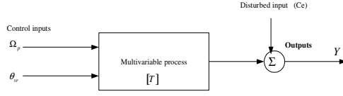
Fig.6. MIMO structure of the process
