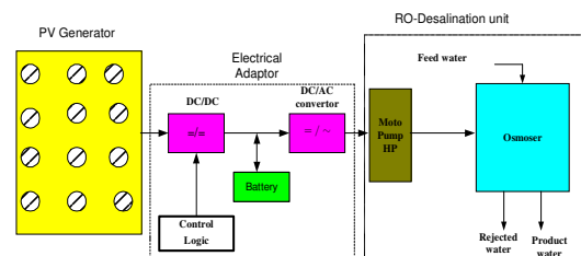
Fig.1. Desalination system coupled to a photovoltaic generator
