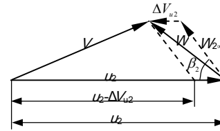
Fig. 6 Velocity triangle at impeller exit
