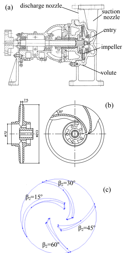
Fig. 1. Pump cross-sectional view (a), impeller style (b) and blade pattern (c)
