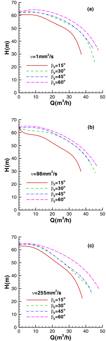
Fig. 2 Head curves in terms of flow rate at three viscosity values
