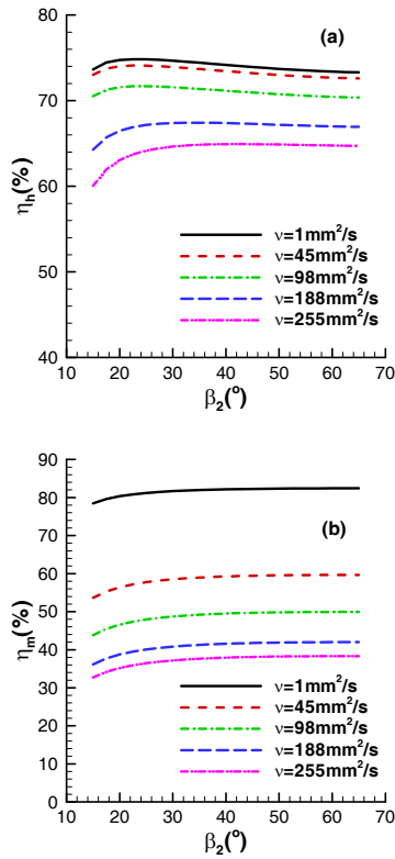
Fig. 10 Estimated hydraulic (a) and mechanical (b) efficiencies at duty point in terms of blade exit angle
