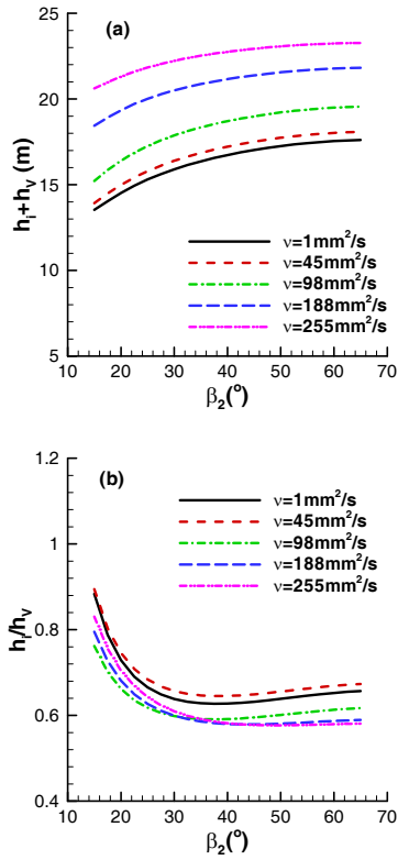
Fig. 14 Ratio of hydraulic losses in impeller to those in volute at BEP in terms of blade discharge angle
