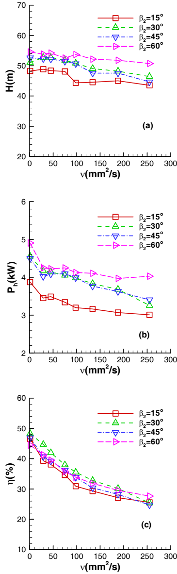
Fig. 5 Head (a), hydraulic power (b) and efficiency (c) at BEP in terms of viscosity
