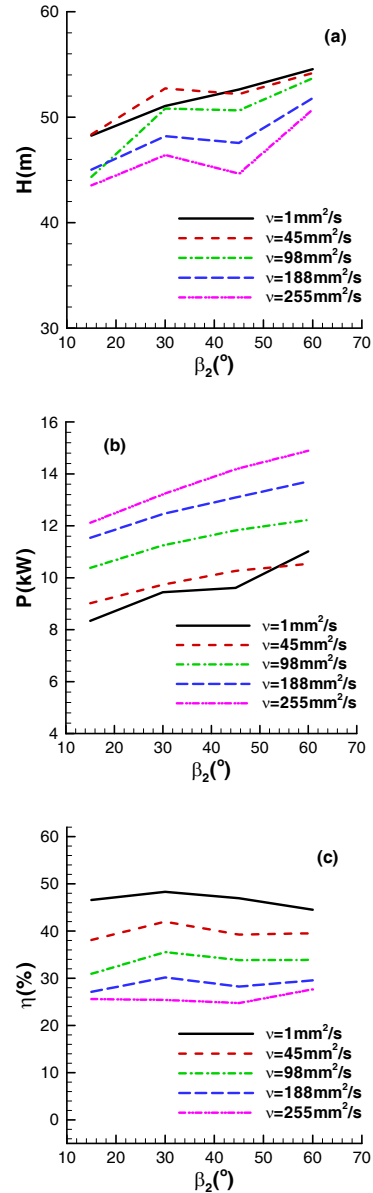
Fig. 9 Experimental head (a), shaft-power (b) and efficiency (c) at duty point in terms of blade exit angle
