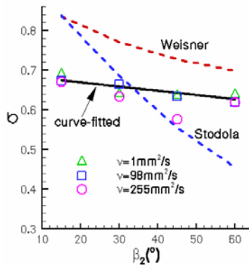
Fig. 7 Slip factor as a function of blade exit angle at three viscosity values at BEP
