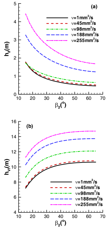
Fig. 11 Hydraulic losses in impeller (a) and volute (b) at duty point in terms of blade discharge angle
