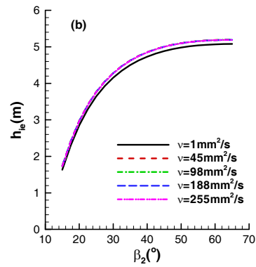
Fig. 13 Estimated diffusion (a) and sudden expansion as well as mixing losses (b) at BEP in terms of blade exit angle
