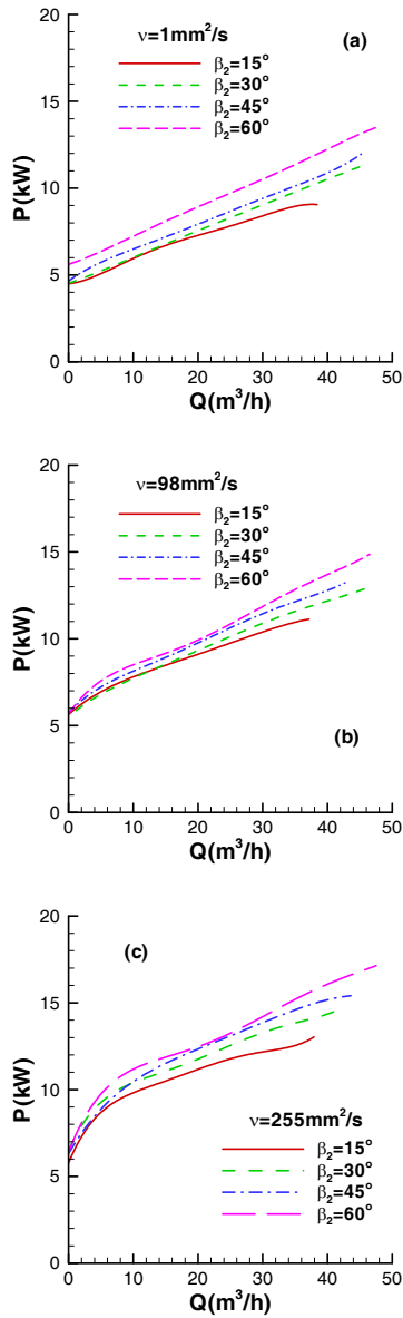
Fig. 3 Shaft-power curves in terms of flow rate at three viscosity values
