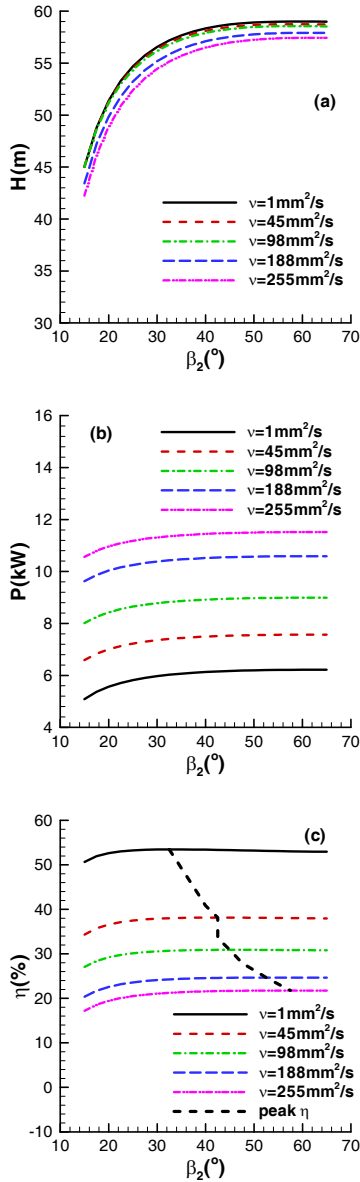
Fig. 8 Computed head (a), shaft-power (b) and efficiency (c) at duty point in terms of blade exit angle
