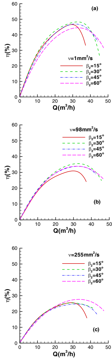
Fig. 4 Efficiency curves against flow rate at three viscosity values
