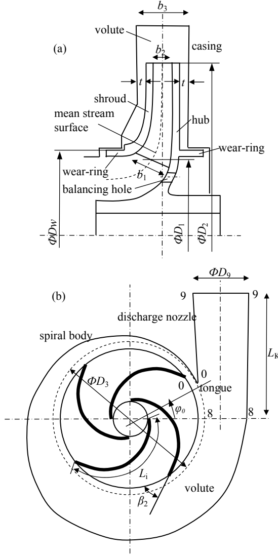
Fig. 7 Major dimensions of impeller (a) and volute (b)
