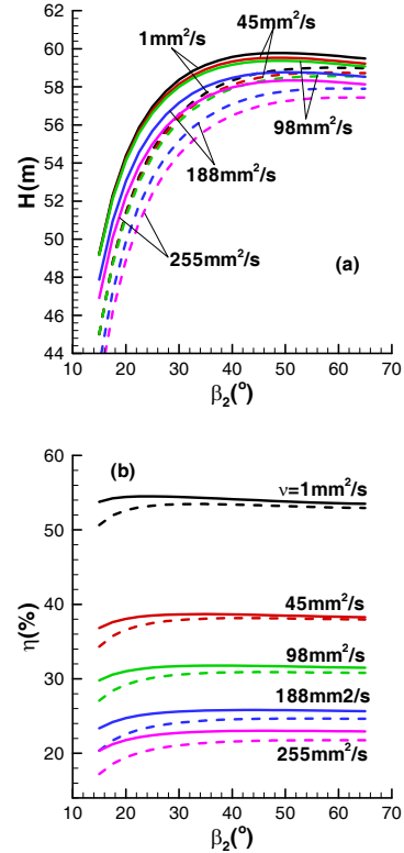
Fig. 15 Comparison of head (a) and efficiency (b) between original and redesigned cases, solid line is for redesigned case and dashed line is for original case
