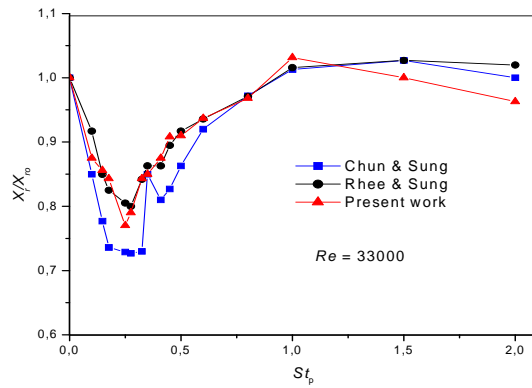
Fig. 4 Normalized reattachment length X_r/X_{r0} against St_p . Re = 33000 , A = 0.3U_0
