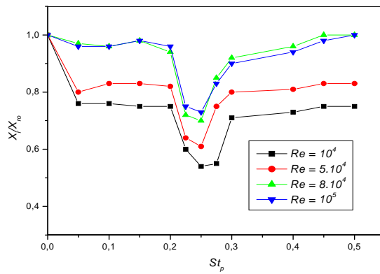
Fig. 5 Normalized reattachment length X_r/X_{r0} against St_p for different Reynolds numbers.
