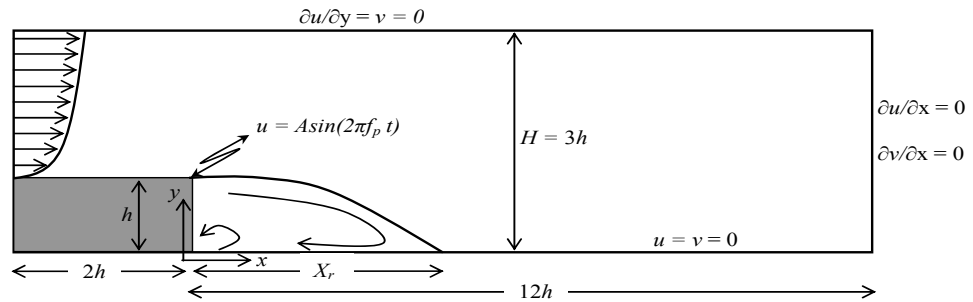
Fig. 1 Geometric configuration of computational domain.
