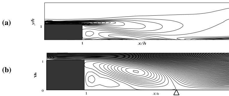
Fig. 2 Distributions of: (a) Iso-vorticity lines, (b) Iso-stream function lines. Re=33000 , without perturbation.
