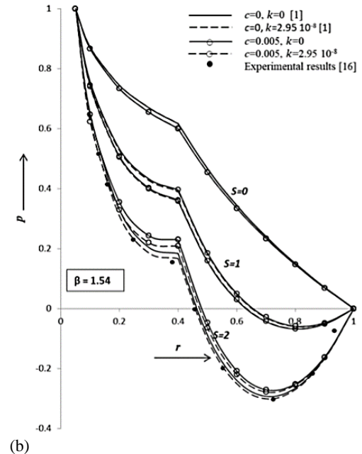
Fig. 3. Variation of film pressure with radius for values of inertia S = 0, 1, 2 and roughness parameter ( c ). (a) Radial Roughness (b) Circumferential Roughness.
