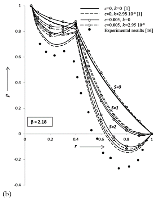
Fig. 2. Variation of film pressure with radius for inertia S = 0, 1, 2 and roughness parameter ( c ). (a) Radial Roughness (b) Circumferential Roughness.
