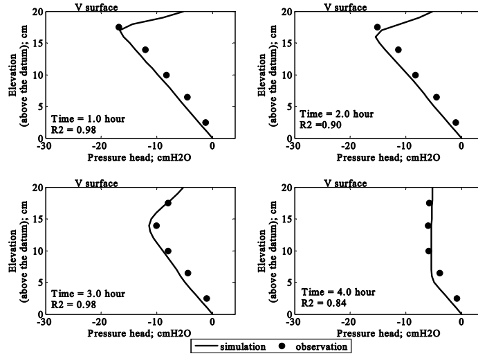
Fig. 5. Pressure head profiles of sand column test.
