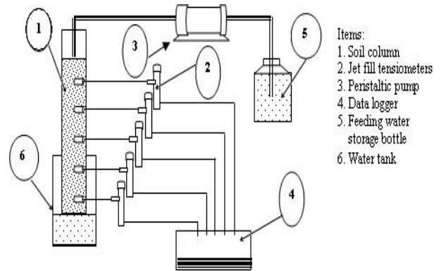
Fig. 1. Column setup.
