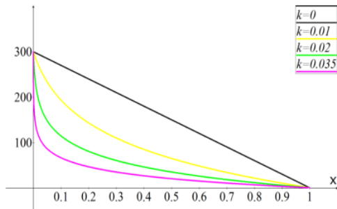
Fig. 2. Plots of p_B(k = 0) and p_{eff} for various values of k > 0 .
