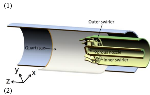
Fig. 2. Setup of swirlers and fuel nozzle.
