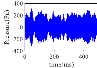
Fig. 12. Dynamic pressure under self-excited combustion instability.
