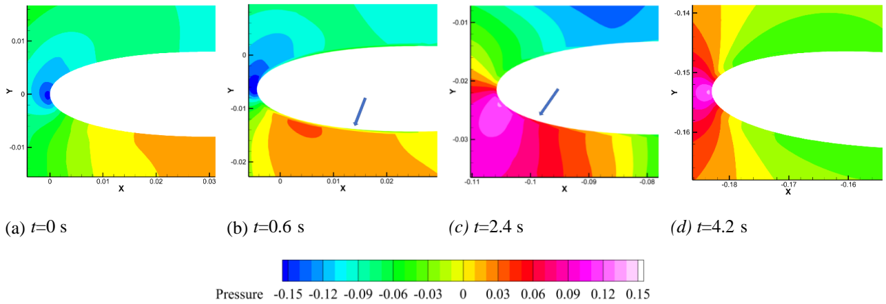
Fig. 16 Pressure cloud during motion of porous airfoil ( \alpha=4\times 10^{-12} , \varepsilon=0.8 )
