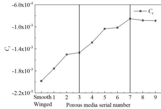
Fig. 3 NACA0016 Traction of various porous wing types
