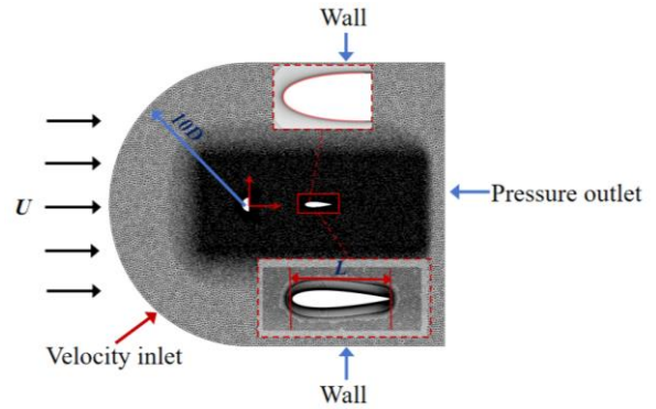
Fig. 1 Grid Partitioning Diagram
