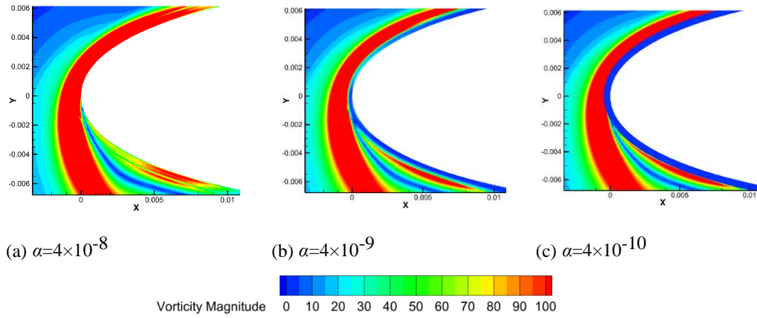
Fig. 6 Leading edge vorticity plots at C_{t,max} for three airfoils with \varepsilon = 0.8 porous media
