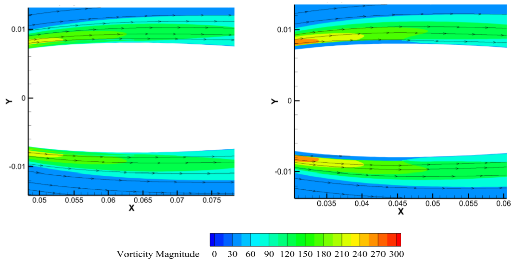
Fig. 5 Vortex cloud and streamline diagrams of two porous airfoil types
