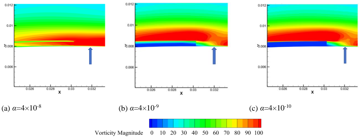
Fig. 7 Plots of vorticity at the end of the porous region at C_{t,max} for three airfoils with \varepsilon = 0.8 porous media
