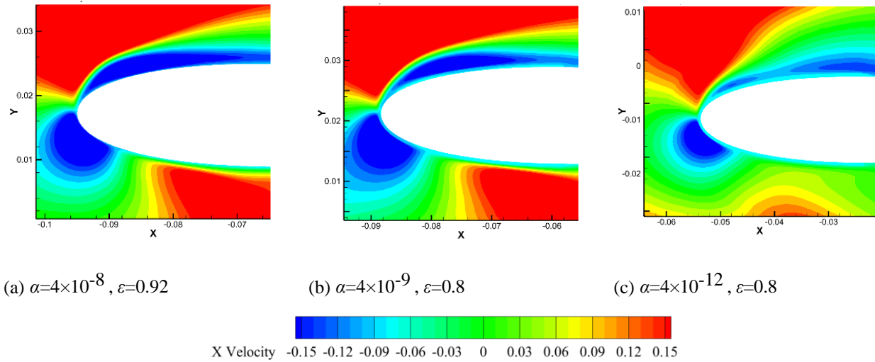
Fig. 15 Horizontal velocity cloud for variable permeability porous airfoils
