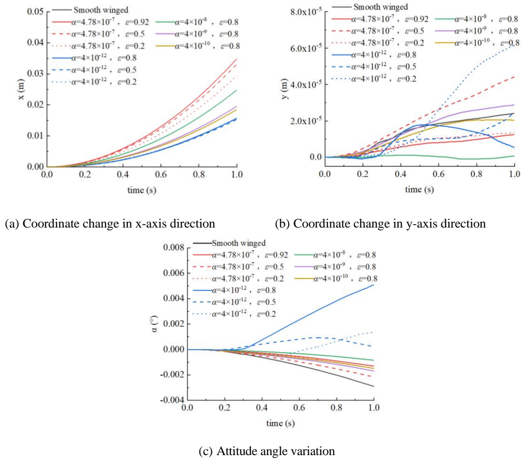
Fig. 4 Variation of Coordinates and Attitude Angle of Various Porous Airfoils for NACA0016 in Incoming Flow Condition
