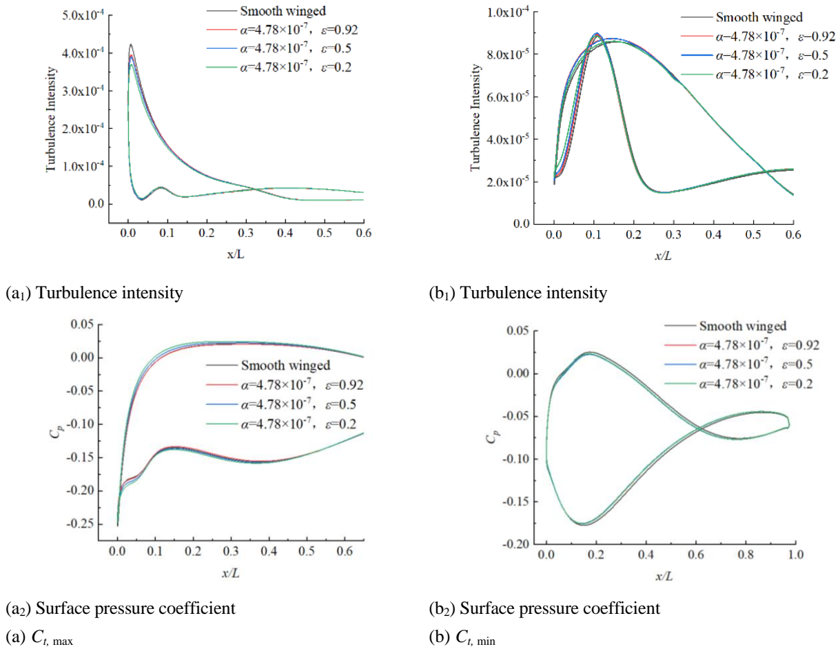
Fig. 9 Airfoil turbulence intensity and surface pressure coefficients for three \alpha = 4.78 \times 10^{-7} porous media
