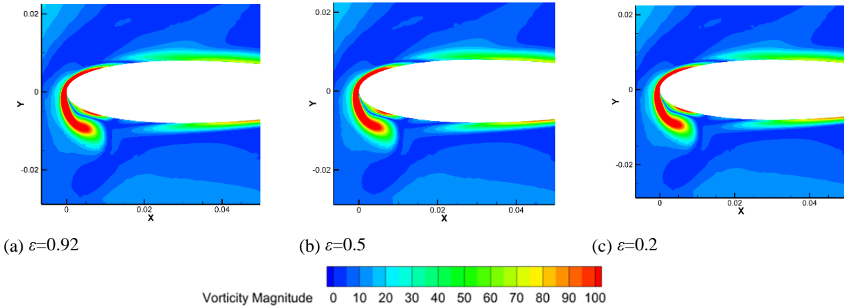
Fig. 8 Vortex profiles at the leading edge of the airfoil at C_{t,max} for three \alpha = 4.78 \times 10^{-7} porous media
