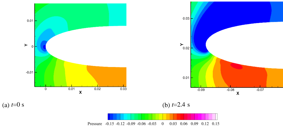
Fig. 17 Pressure cloud during motion of porous airfoil ( \alpha = 4 \times 10^{-9} , \varepsilon = 0.8 )
