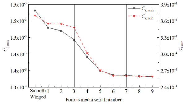
Fig. 11 Maximum Traction Force of Various Porous Media
