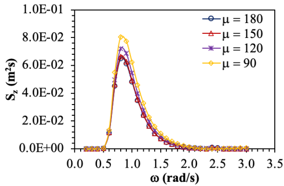
(a) Heave response to irregular waves
