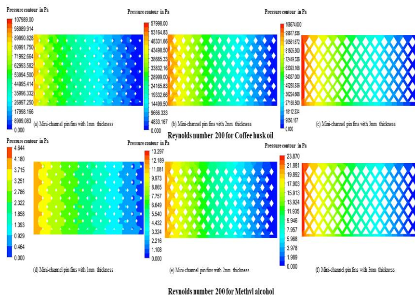
Fig. 12 Pressure contour at Re 200
