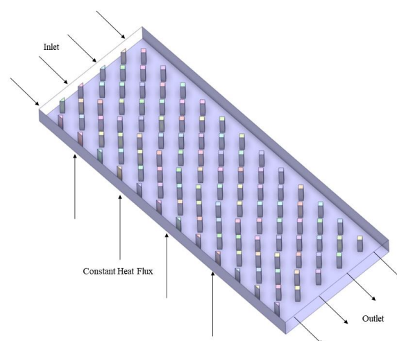
Fig. 2 Computational domain
