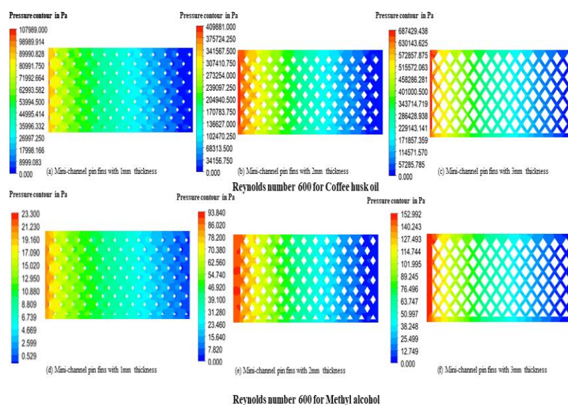
Fig. 13 Pressure contour at Re 600
