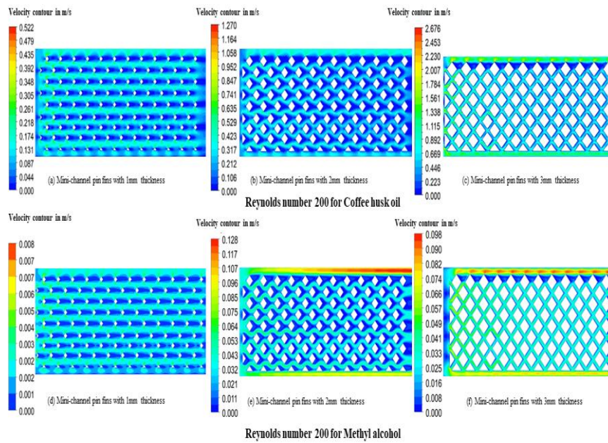
Fig. 14 Velocity contour at Re 200
