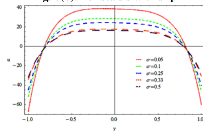
Fig. 6(c). With cilia
